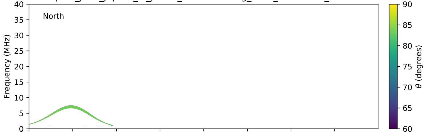
expres_juno_jupiter_io_jrm09_lossc-wid1deg_3kev_20190722_v01.cdf
