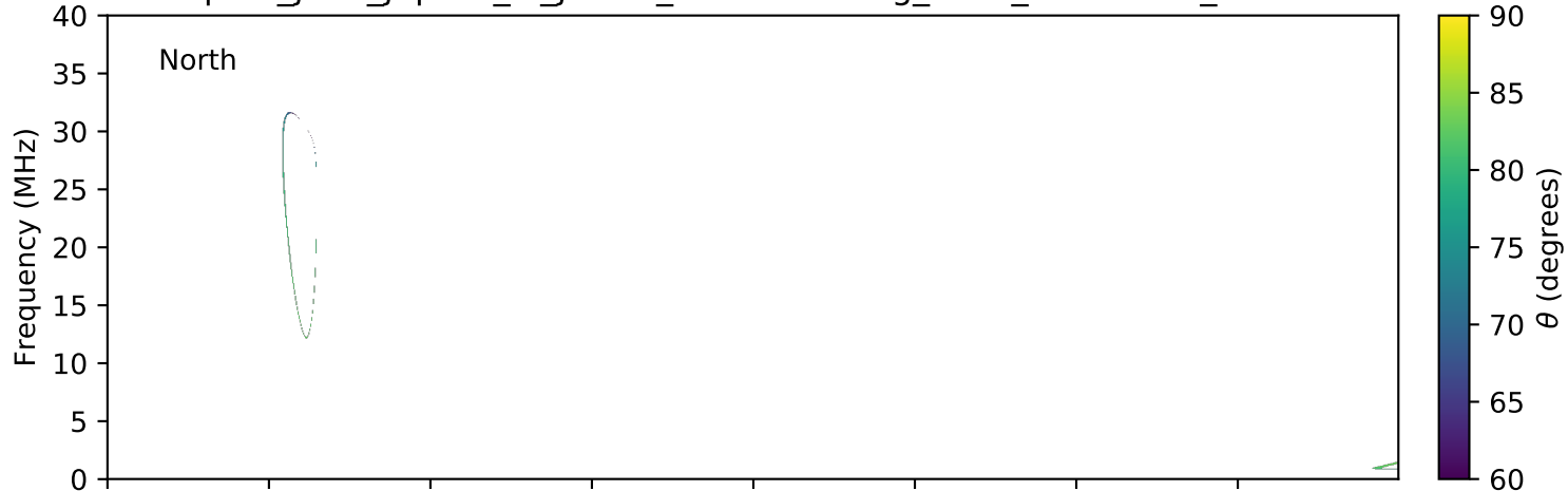
expres_juno_jupiter_io_jrm09_lossc-wid1deg_3kev_20190721_v01.cdf
