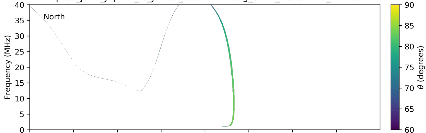
expres_juno_jupiter_io_jrm09_lossc-wid1deg_3kev_20190720_v01.cdf
