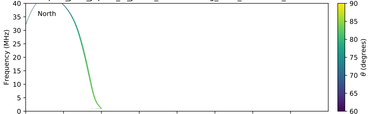
expres_juno_jupiter_io_jrm09_lossc-wid1deg_3kev_20190715_v01.cdf
