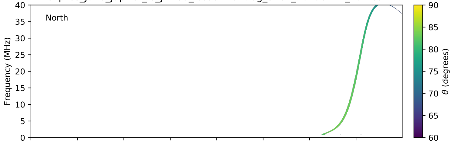
expres_juno_jupiter_io_jrm09_lossc-wid1deg_3kev_20190712_v01.cdf
