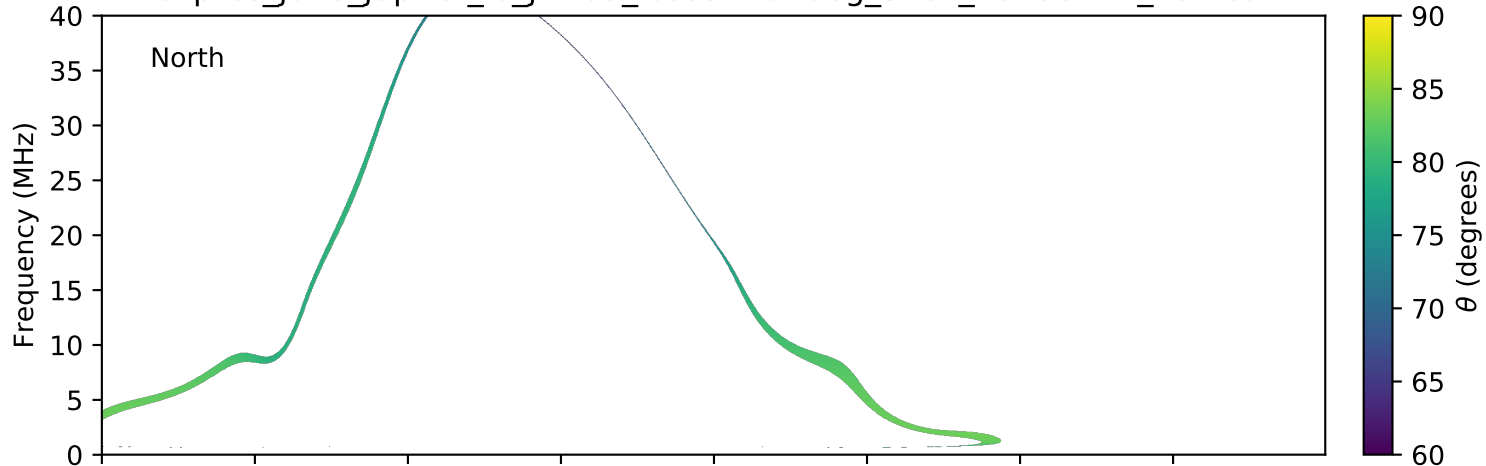
expres_juno_jupiter_io_jrm09_lossc-wid1deg_3kev_20190711_v01.cdf
