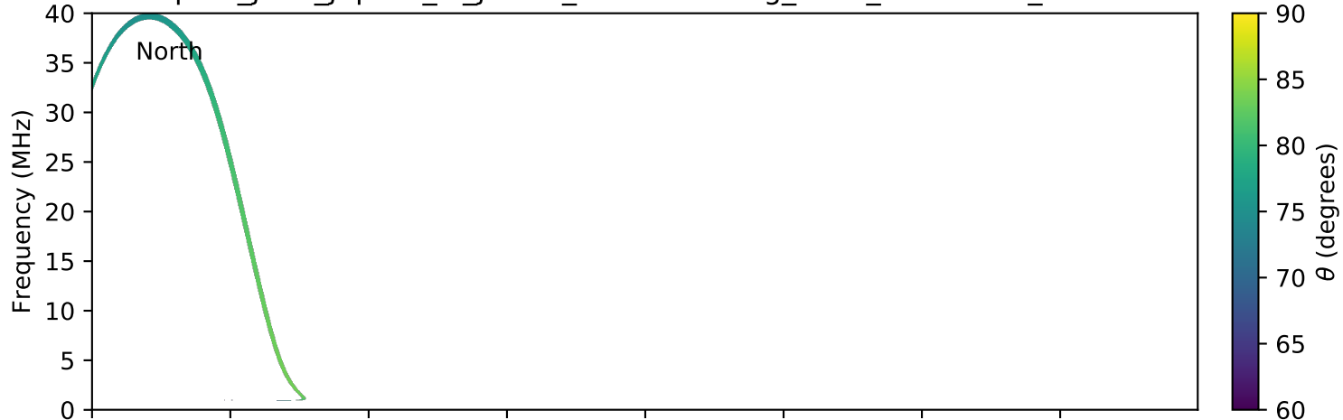
expres_juno_jupiter_io_jrm09_lossc-wid1deg_3kev_20190708_v01.cdf
