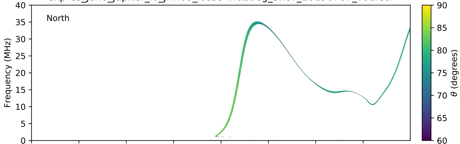
expres_juno_jupiter_io_jrm09_lossc-wid1deg_3kev_20190707_v01.cdf
