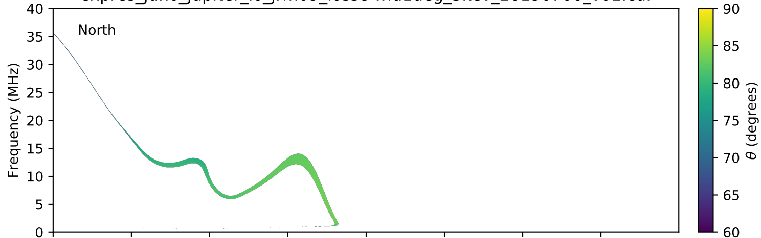
expres_juno_jupiter_io_jrm09_lossc-wid1deg_3kev_20190706_v01.cdf
