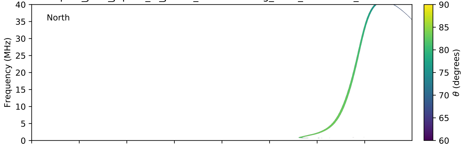
expres_juno_jupiter_io_jrm09_lossc-wid1deg_3kev_20190705_v01.cdf
