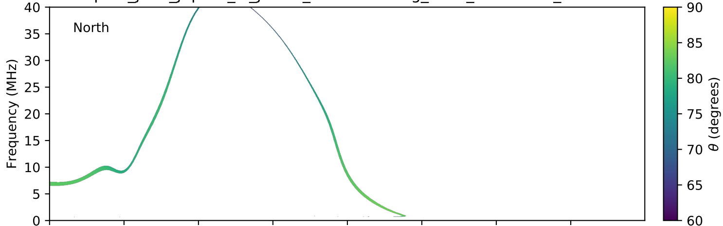
expres_juno_jupiter_io_jrm09_lossc-wid1deg_3kev_20190704_v01.cdf
