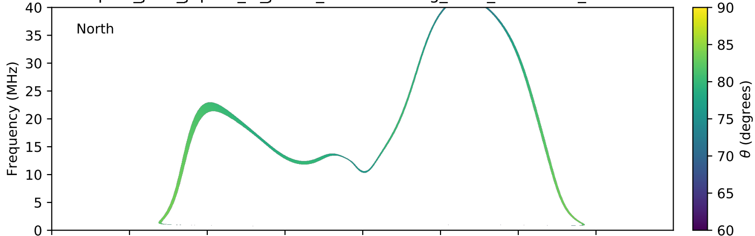
expres_juno_jupiter_io_jrm09_lossc-wid1deg_3kev_20190702_v01.cdf
