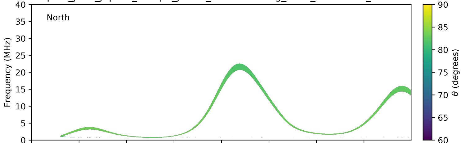
expres_juno_jupiter_europa_jrm09_lossc-wid1deg_3kev_20190729_v01.cdf
