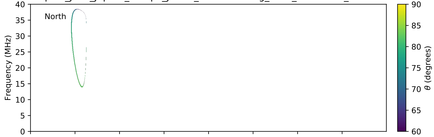
expres_juno_jupiter_europa_jrm09_lossc-wid1deg_3kev_20190721_v01.cdf
