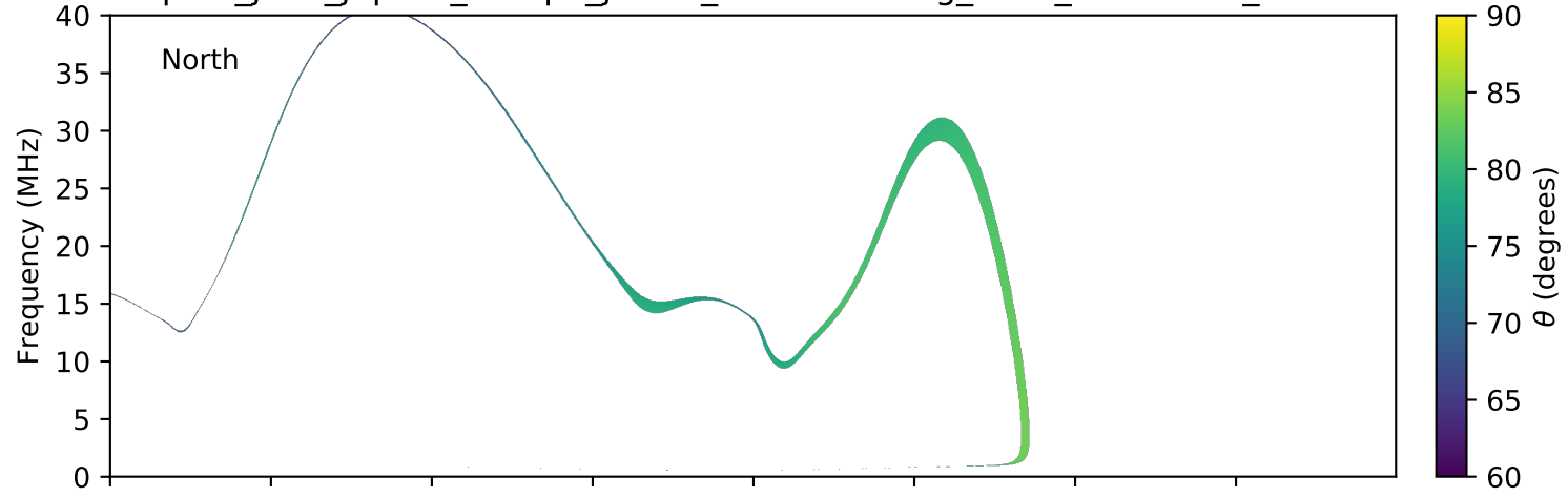
expres_juno_jupiter_europa_jrm09_lossc-wid1deg_3kev_20190719_v01.cdf
