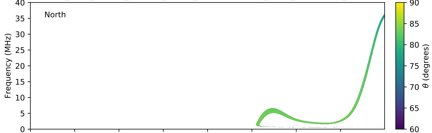
expres_juno_jupiter_europa_jrm09_lossc-wid1deg_3kev_20190714_v01.cdf
