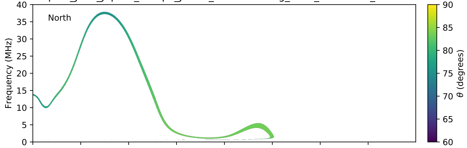
expres_juno_jupiter_europa_jrm09_lossc-wid1deg_3kev_20190712_v01.cdf
