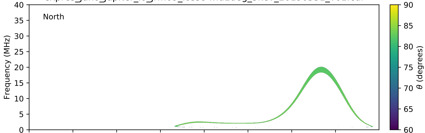
expres_juno_jupiter_io_jrm09_lossc-wid1deg_3kev_20190531_v01.cdf
