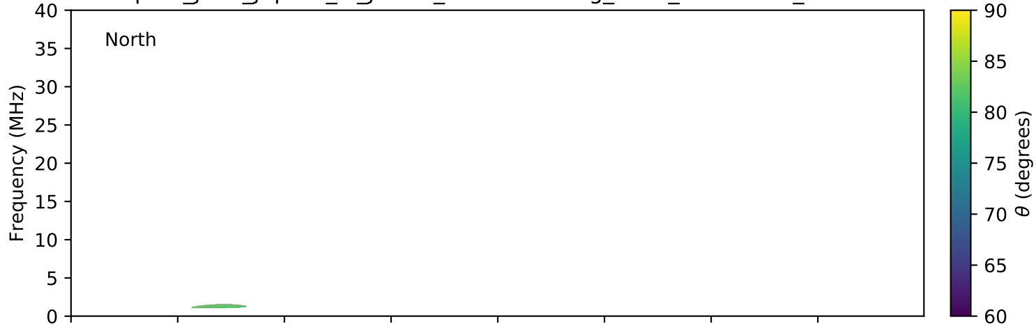
expres_juno_jupiter_io_jrm09_lossc-wid1deg_3kev_20190530_v01.cdf
