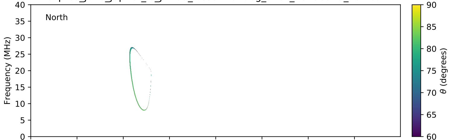
expres_juno_jupiter_io_jrm09_lossc-wid1deg_3kev_20190529_v01.cdf
