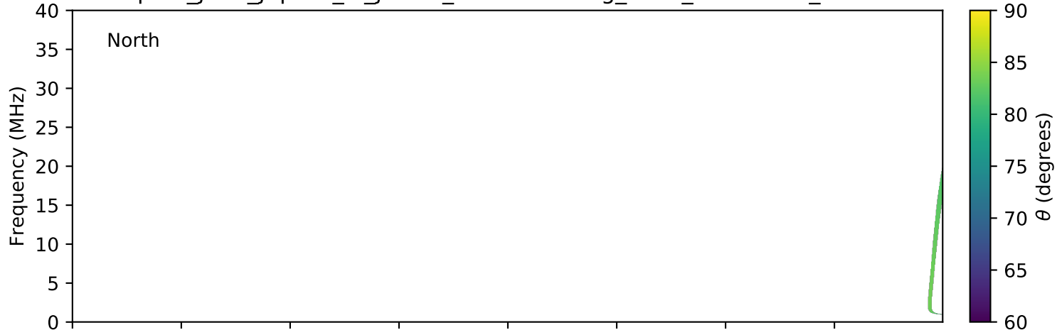
expres_juno_jupiter_io_jrm09_lossc-wid1deg_3kev_20190525_v01.cdf
