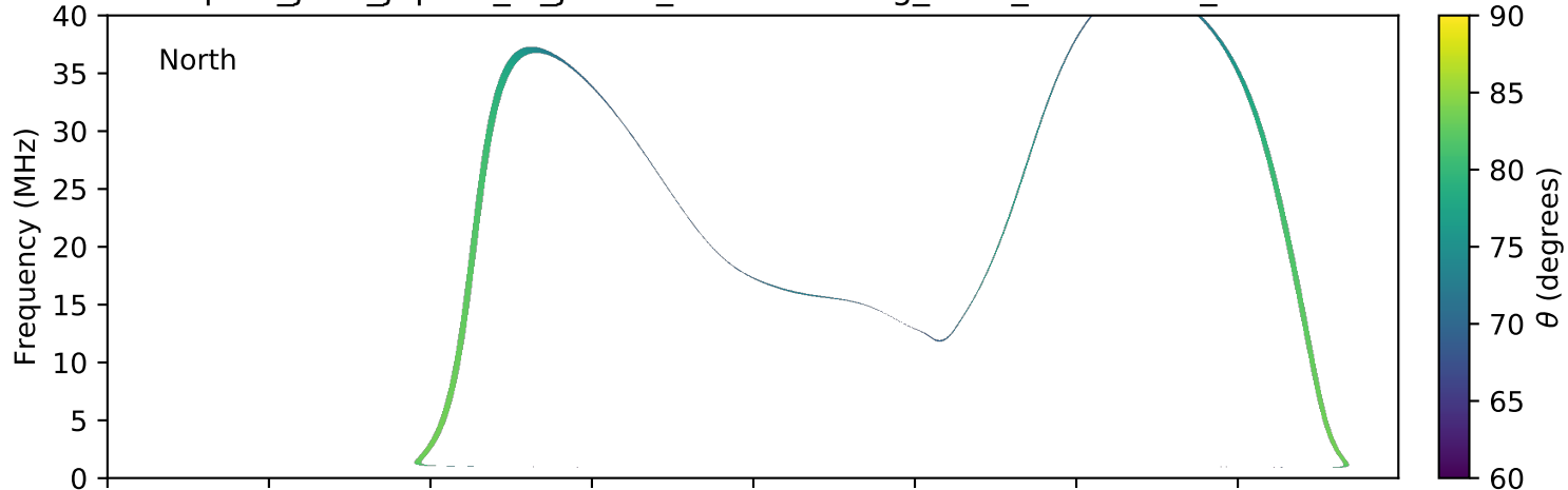
expres_juno_jupiter_io_jrm09_lossc-wid1deg_3kev_20190524_v01.cdf
