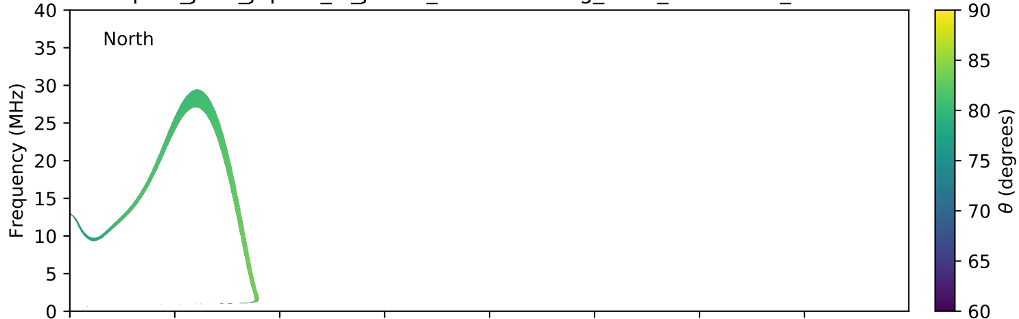
expres_juno_jupiter_io_jrm09_lossc-wid1deg_3kev_20190523_v01.cdf
