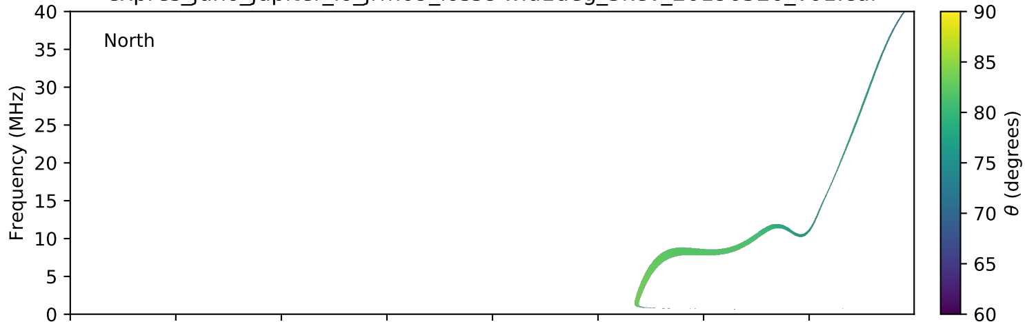
expres_juno_jupiter_io_jrm09_lossc-wid1deg_3kev_20190520_v01.cdf
