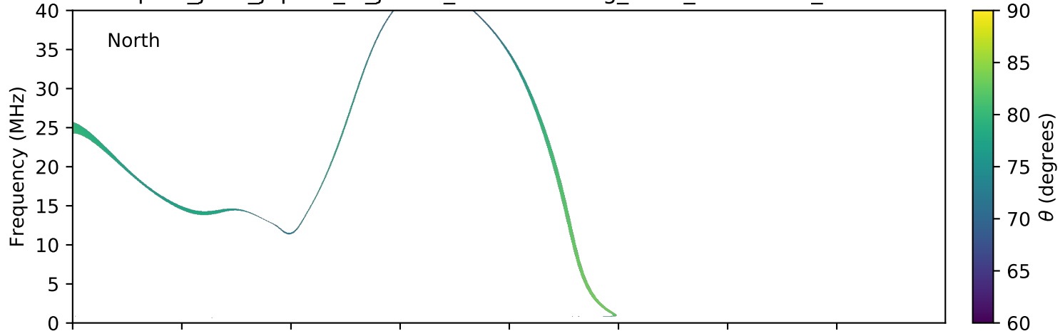
expres_juno_jupiter_io_jrm09_lossc-wid1deg_3kev_20190519_v01.cdf
