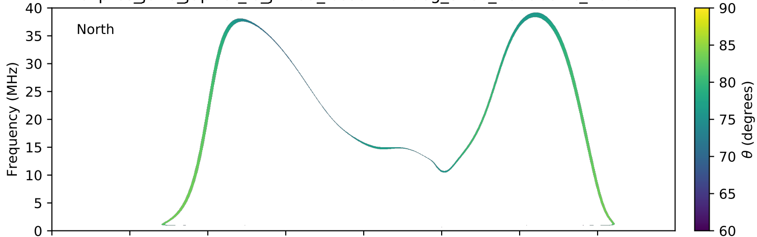
expres_juno_jupiter_io_jrm09_lossc-wid1deg_3kev_20190517_v01.cdf
