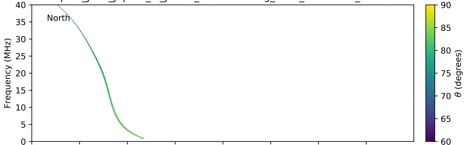
expres_juno_jupiter_io_jrm09_lossc-wid1deg_3kev_20190514_v01.cdf
