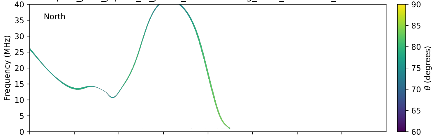
expres_juno_jupiter_io_jrm09_lossc-wid1deg_3kev_20190512_v01.cdf
