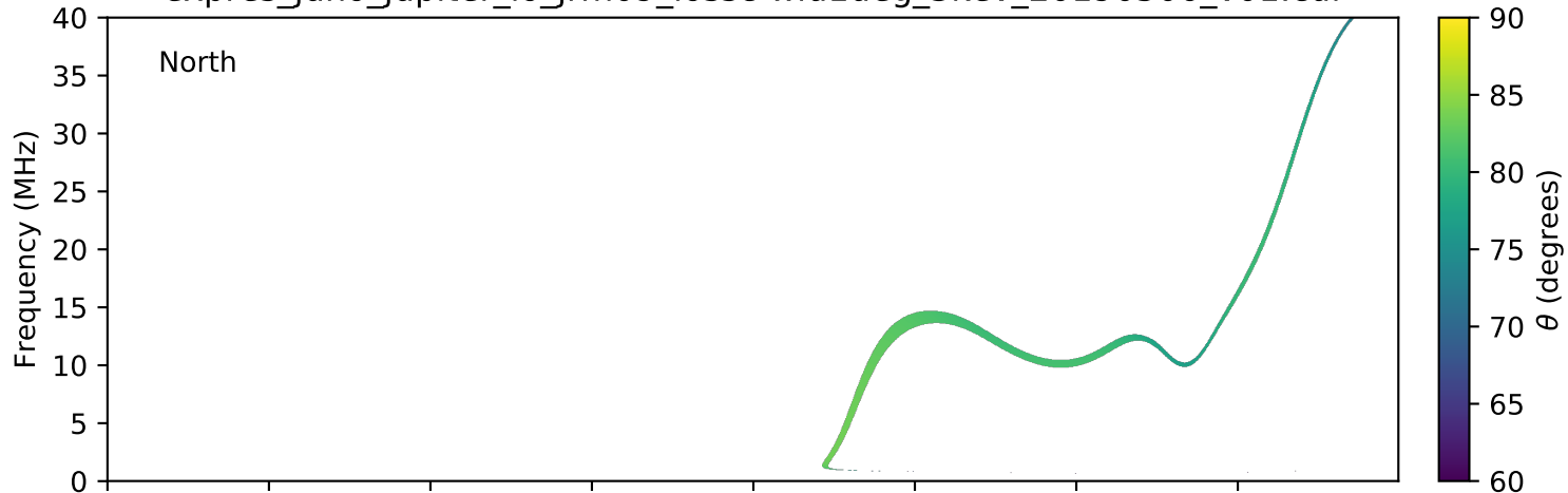
expres_juno_jupiter_io_jrm09_lossc-wid1deg_3kev_20190506_v01.cdf
