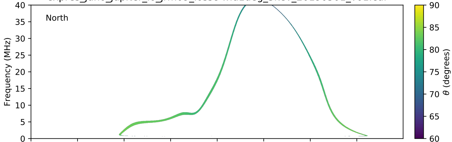
expres_juno_jupiter_io_jrm09_lossc-wid1deg_3kev_20190501_v01.cdf
