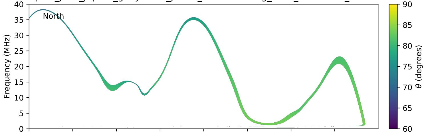
expres_juno_jupiter_ganymede_jrm09_lossc-wid1deg_3kev_20190526_v01.cdf
