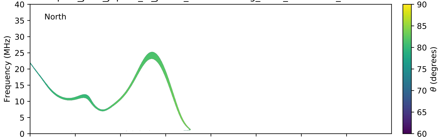
expres_juno_jupiter_io_jrm09_lossc-wid1deg_3kev_20190428_v01.cdf
