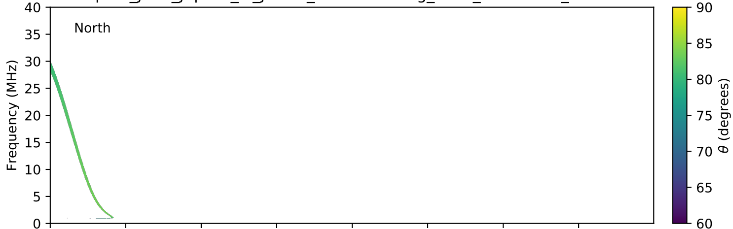
expres_juno_jupiter_io_jrm09_lossc-wid1deg_3kev_20190423_v01.cdf
