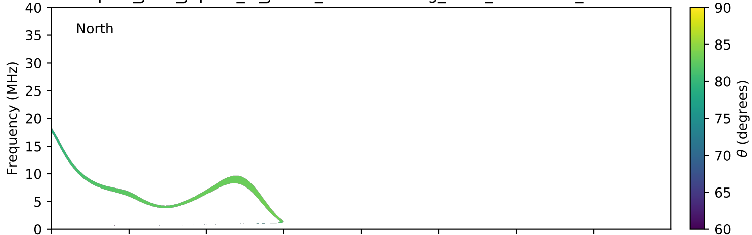
expres_juno_jupiter_io_jrm09_lossc-wid1deg_3kev_20190421_v01.cdf
