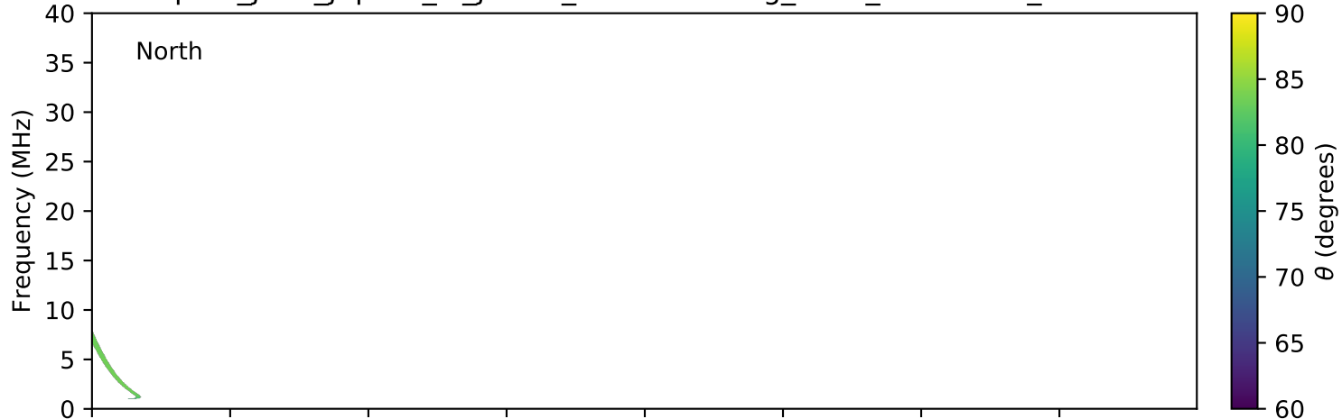
expres_juno_jupiter_io_jrm09_lossc-wid1deg_3kev_20190416_v01.cdf
