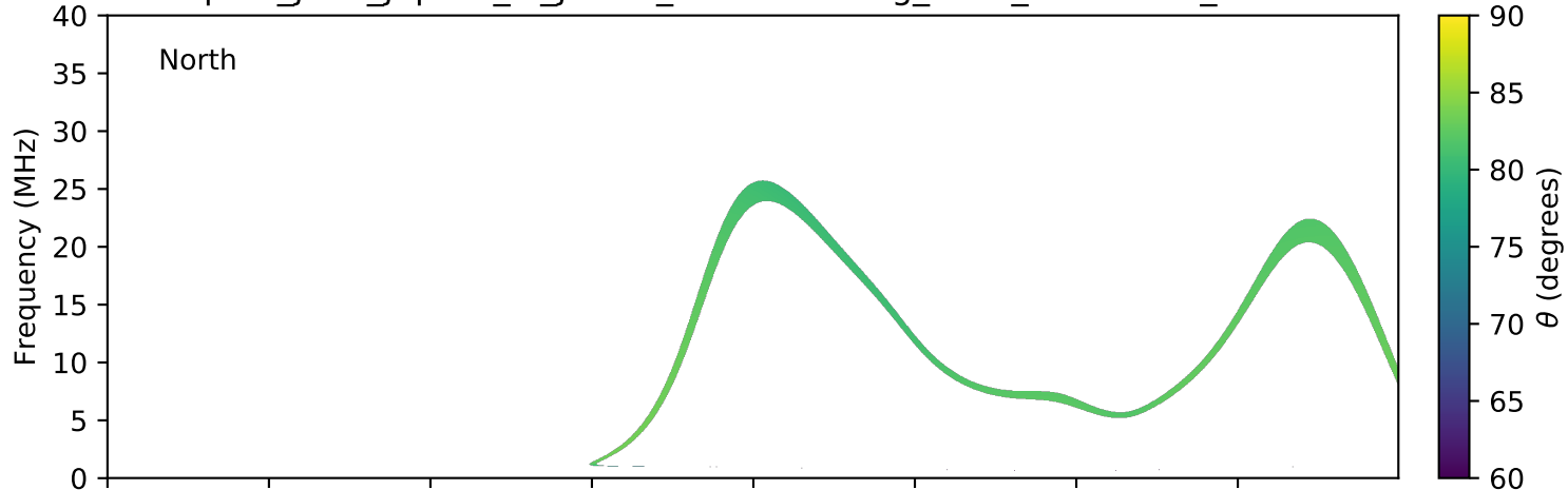
expres_juno_jupiter_io_jrm09_lossc-wid1deg_3kev_20190415_v01.cdf
