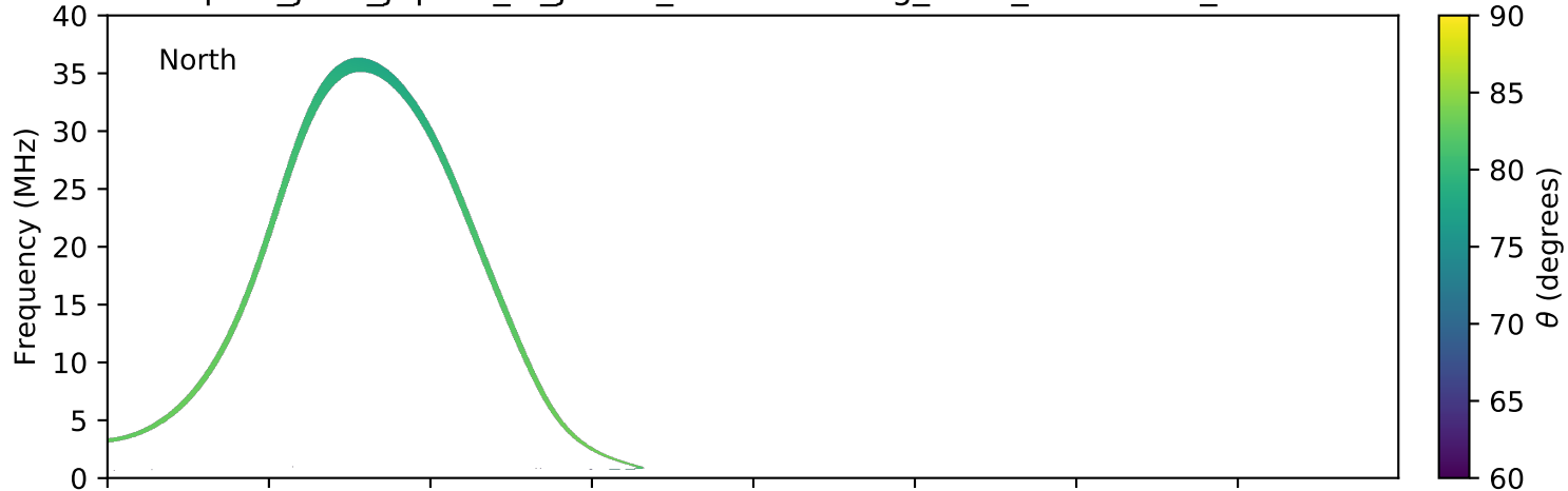
expres_juno_jupiter_io_jrm09_lossc-wid1deg_3kev_20190412_v01.cdf
