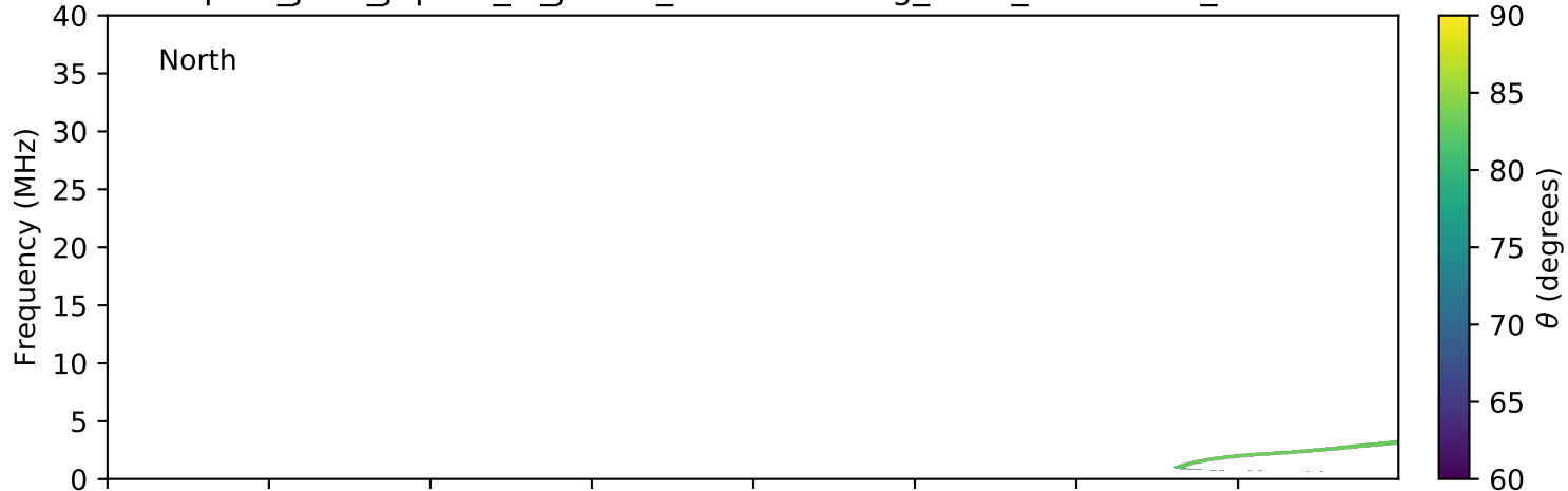
expres_juno_jupiter_io_jrm09_lossc-wid1deg_3kev_20190411_v01.cdf
