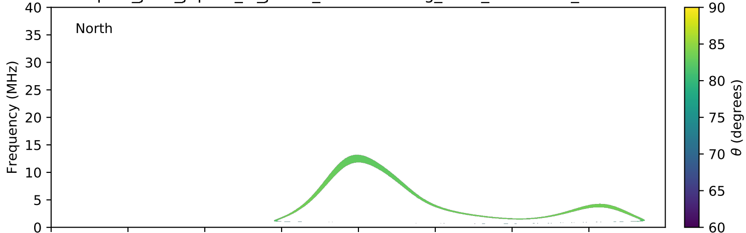
expres_juno_jupiter_io_jrm09_lossc-wid1deg_3kev_20190408_v01.cdf
