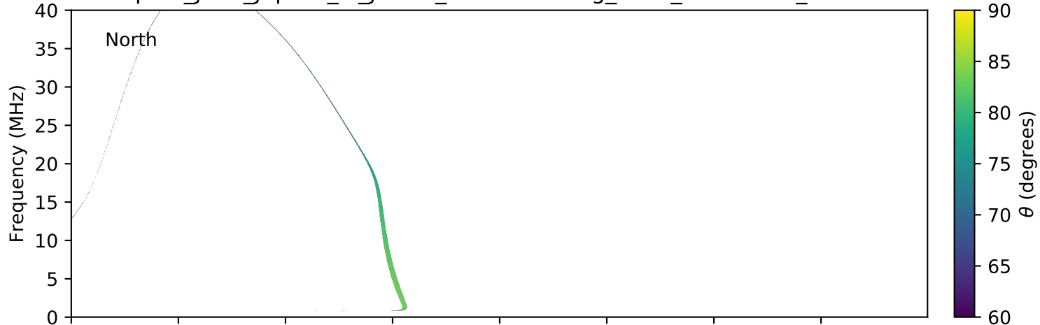
expres_juno_jupiter_io_jrm09_lossc-wid1deg_3kev_20190405_v01.cdf
