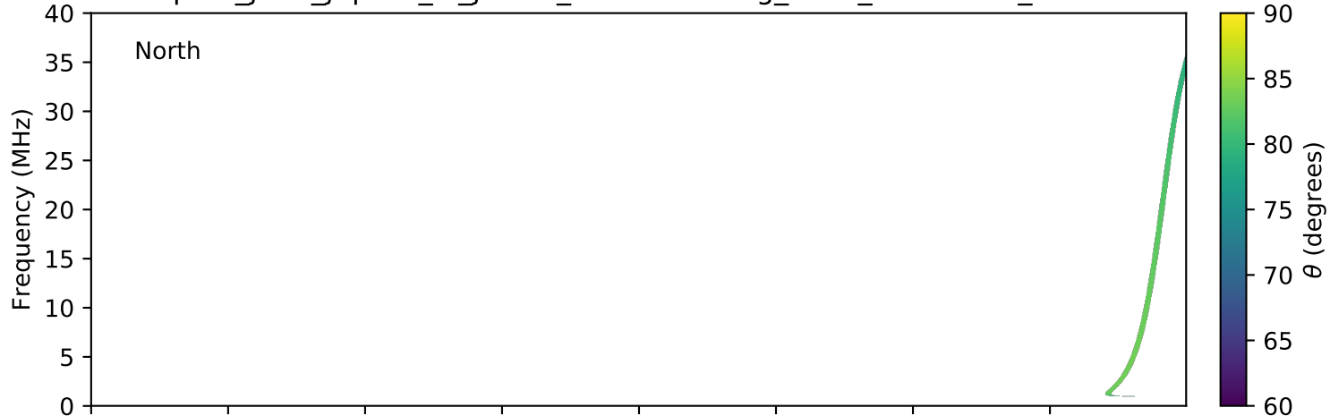
expres_juno_jupiter_io_jrm09_lossc-wid1deg_3kev_20190402_v01.cdf
