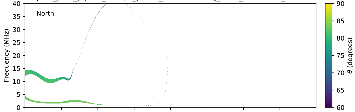
expres_juno_jupiter_europa_jrm09_lossc-wid1deg_3kev_20190406_v01.cdf
