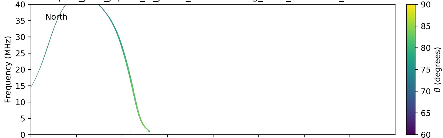
expres_juno_jupiter_io_jrm09_lossc-wid1deg_3kev_20190329_v01.cdf
