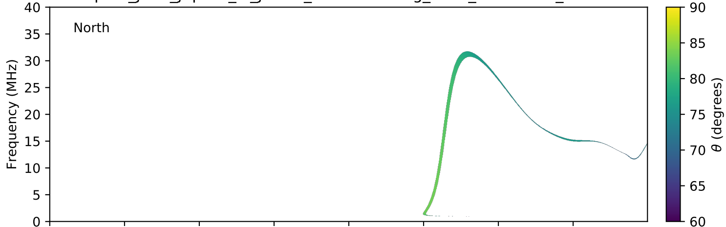
expres_juno_jupiter_io_jrm09_lossc-wid1deg_3kev_20190328_v01.cdf
