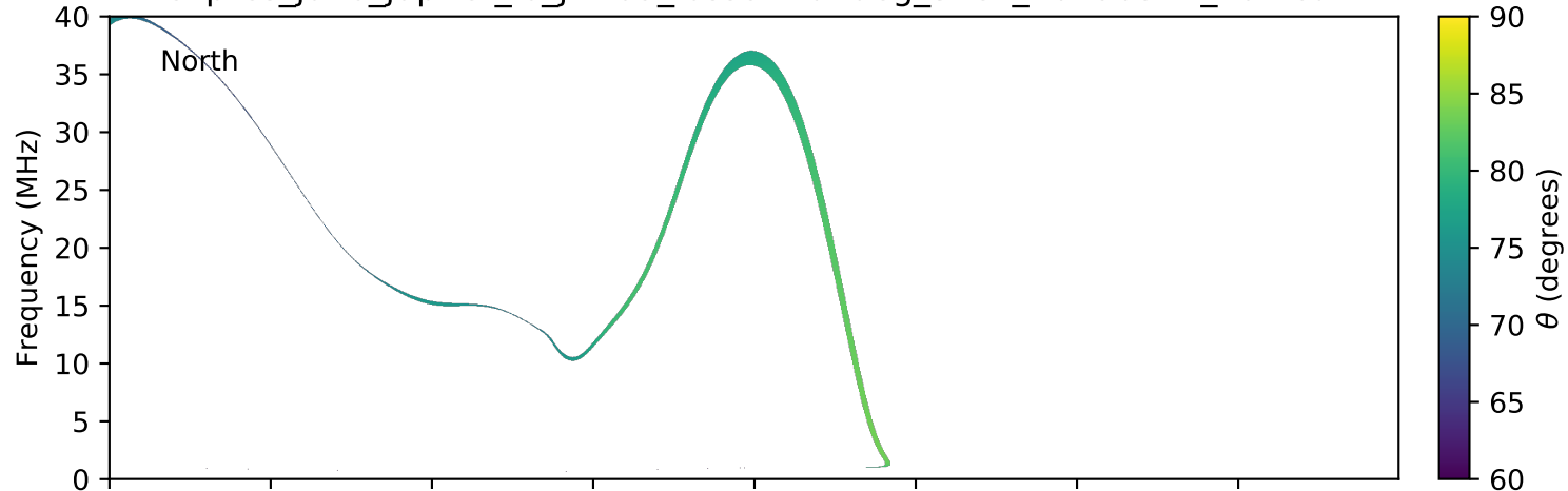
expres_juno_jupiter_io_jrm09_lossc-wid1deg_3kev_20190327_v01.cdf
