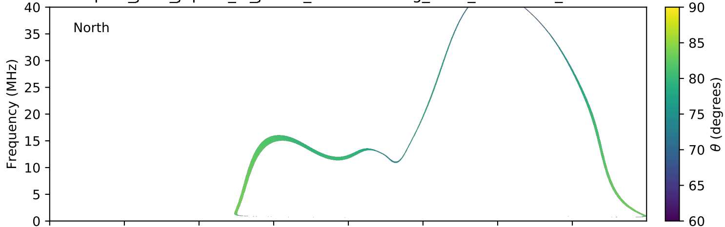
expres_juno_jupiter_io_jrm09_lossc-wid1deg_3kev_20190323_v01.cdf
