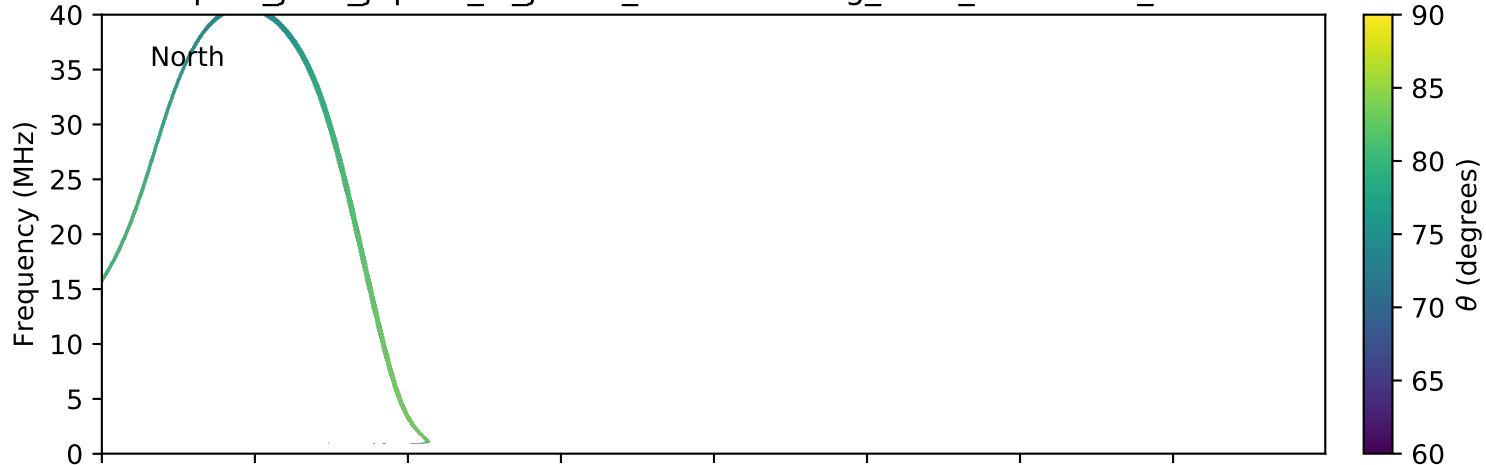
expres_juno_jupiter_io_jrm09_lossc-wid1deg_3kev_20190322_v01.cdf
