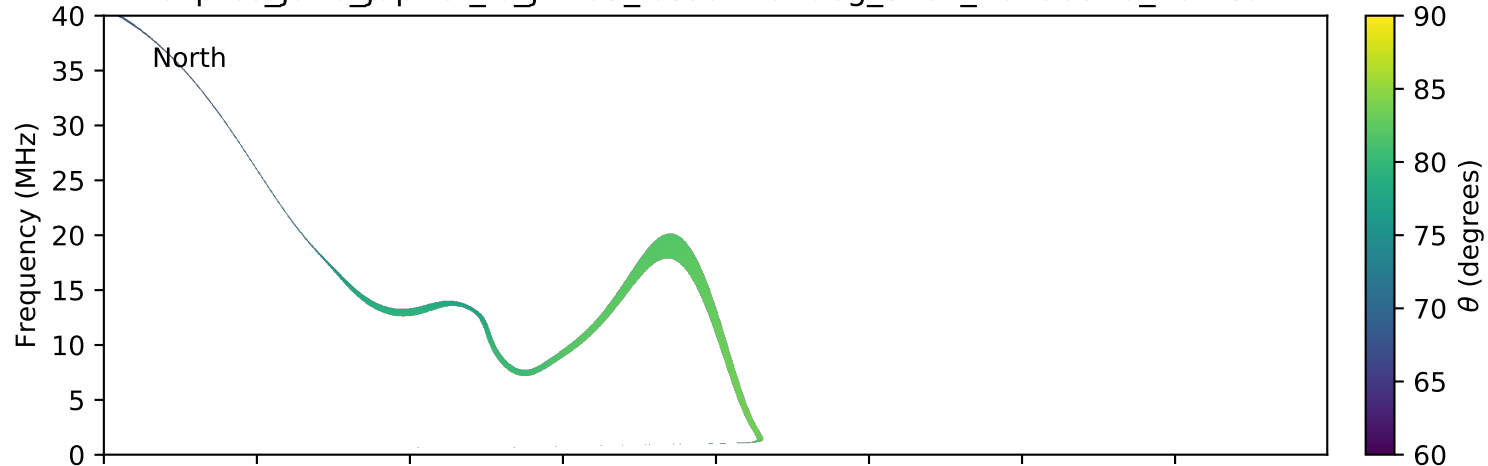
expres_juno_jupiter_io_jrm09_lossc-wid1deg_3kev_20190320_v01.cdf
