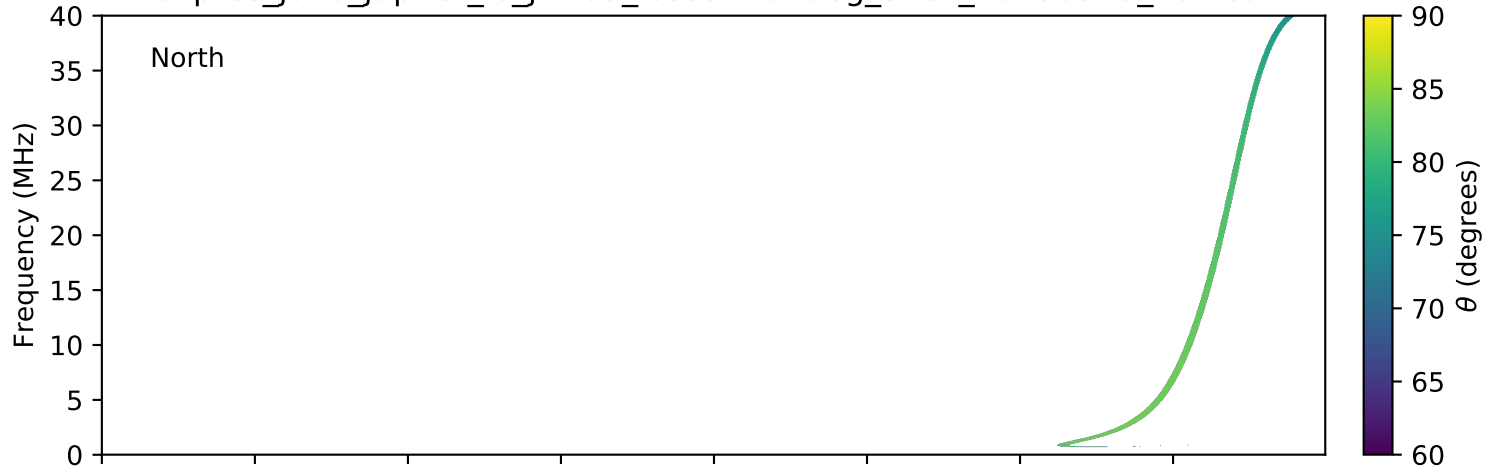
expres_juno_jupiter_io_jrm09_lossc-wid1deg_3kev_20190319_v01.cdf
