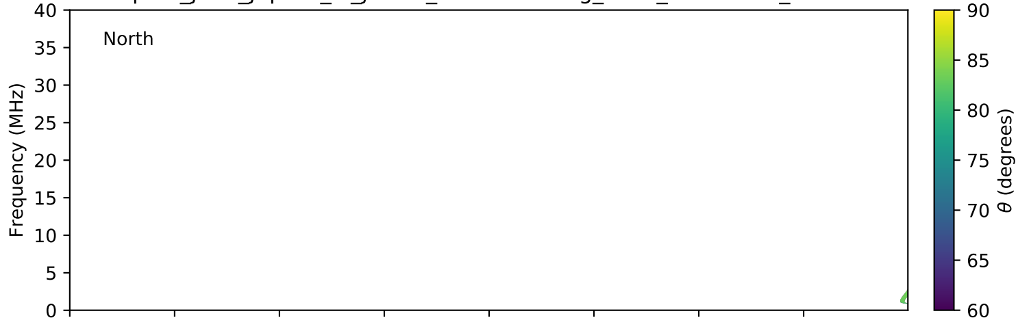
expres_juno_jupiter_io_jrm09_lossc-wid1deg_3kev_20190317_v01.cdf
